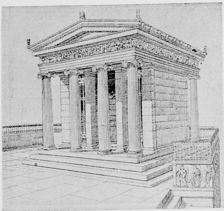
Ὁ ναὸς τῆς Ἀθηνᾶς (Ἀπτέρου) Νίκης, ἰωνικοῦ ρυθμοῦ (Ἀναπαράστασις)
